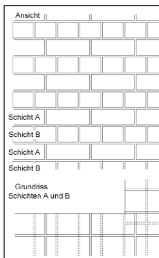
Blockverband
